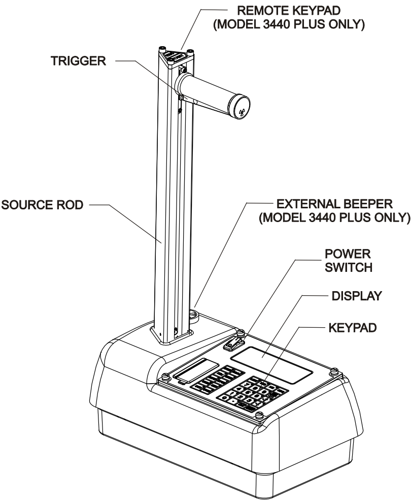
Figure 3–1. Gauge Illustration
