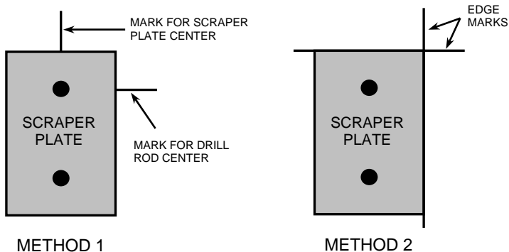
Figure 4-3. Marking the Test Area
